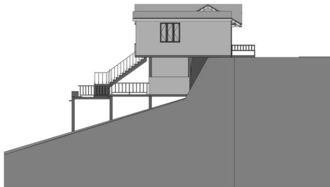
West Elevation
